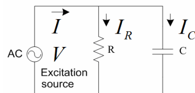
Figure 1: Equivalent circuit for \text{Tan } \delta measurements
